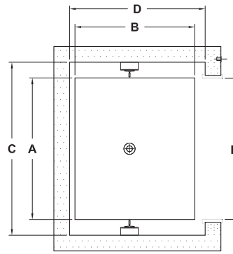
FRONT OPENING
